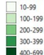
incidence rate: past 14 days per 100000
