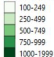
incidence rate: cumulative per 100000
